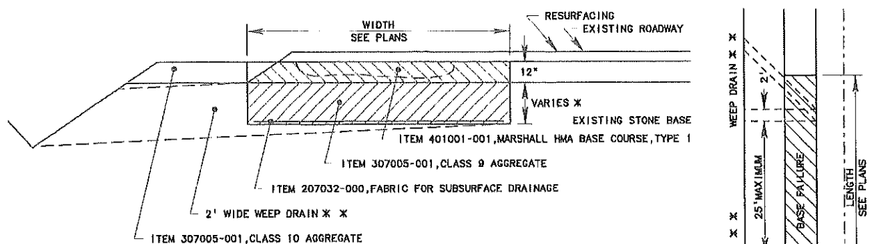
(ELEVATION VIEW)
