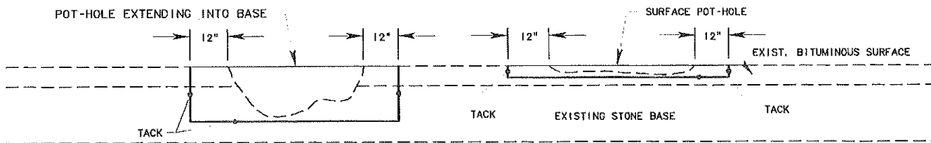
(ELEVATION VIEW)
