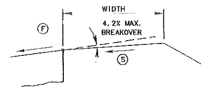
SUPERELEVATED SECTIONS-HIGH SIDE
